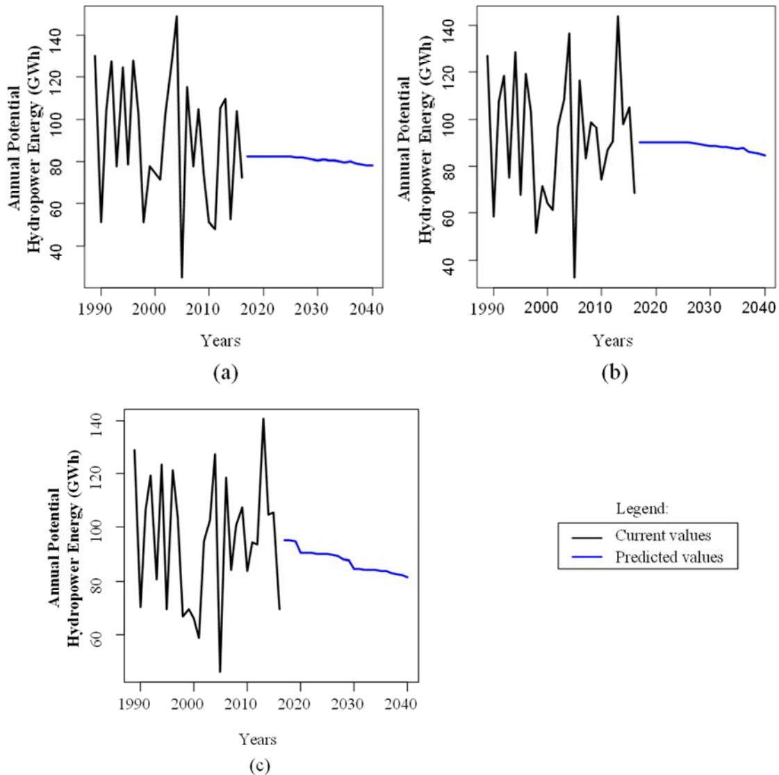
Figure 8. Annual potential hydropower energy over time for periods of 1989-2016 and 2017-2040 at Savè site. (a) Case of a Single turbine of 90 m³/s; (b) Case of Double turbines of 45 m³/s; (c) Case of Triple turbines of 30 m³/s.
