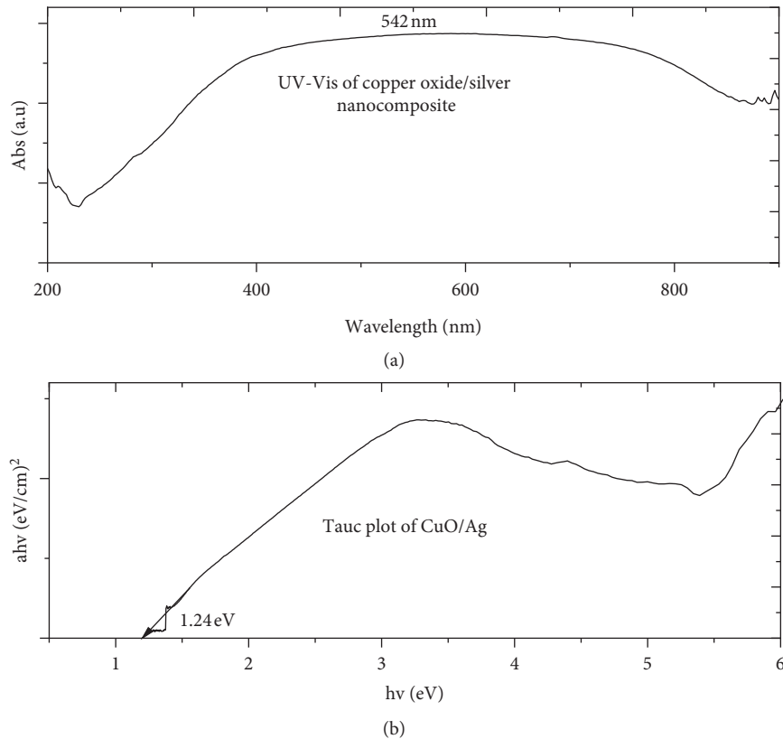
FIGURE 5: (a) UV-Vis spectrophotometric absorption spectra of CuO/Ag and (b) Tauc plot of CuO/Ag.
