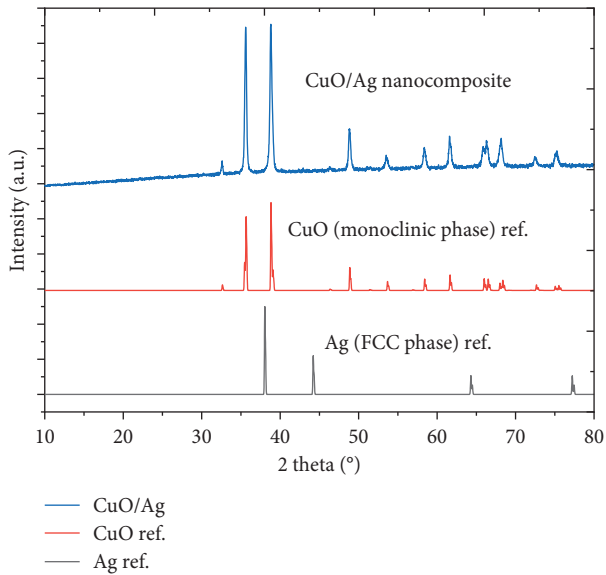
FIGURE 1: XRD spectrum of CuO/Ag correlated with the reference data of CuO monoclinic phase and the face centered cubic (FCC) phase of Ag.
