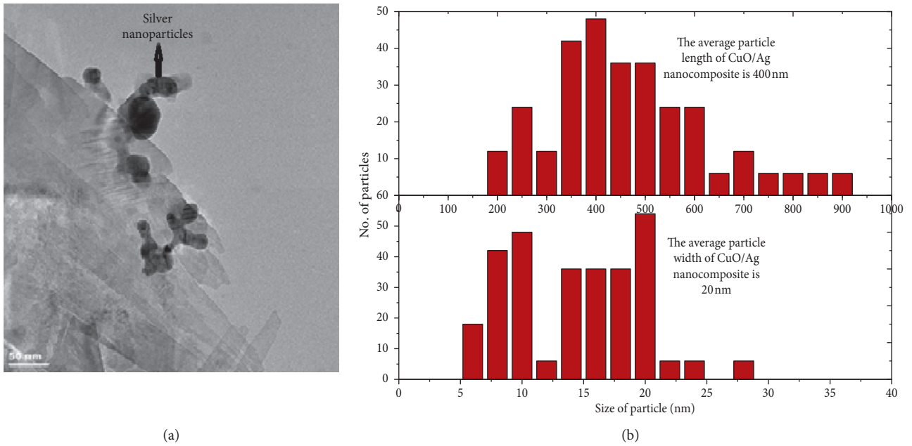
FIGURE 3: (a) TEM micrograph of CuO/Ag. (b) Particle size distribution of CuO/Ag nanocomposite.
