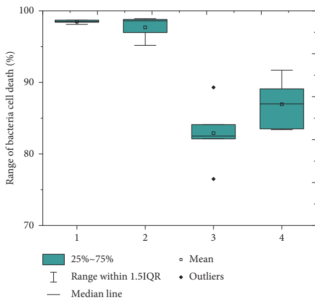
FIGURE 21: A boxplot of the antibacterial activities of nanocomposites (CuO/Ag and ZnO/Ag) against bacteria species. 1 = CuO/Ag against E. coli , 2 = CuO/Ag against S. aureus , 3 = ZnO/Ag against E. coli , and 4 = ZnO/Ag against S. aureus .
