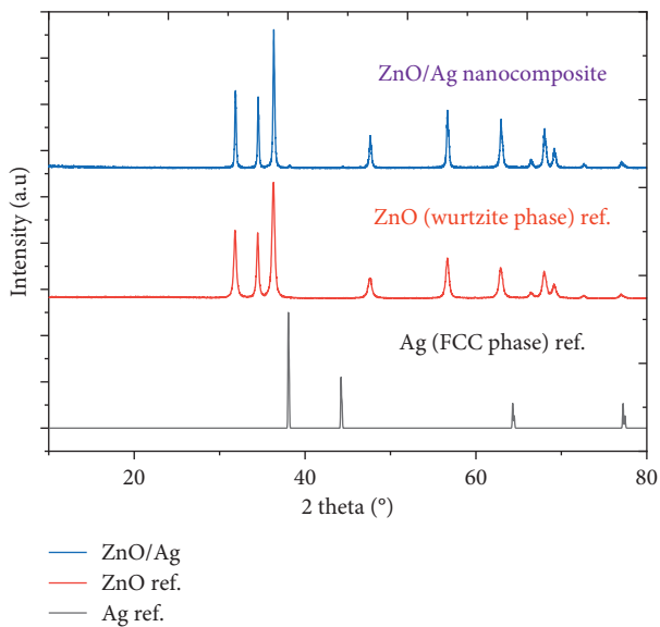
FIGURE 2: XRD pattern of ZnO/Ag nanocomposite in correlation with the wurtzite phase of ZnO and the face centered cubic (FCC) phase of Ag.
