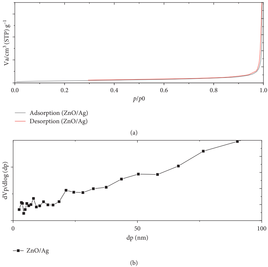
FIGURE 8: (a) Adsorption-desorption isotherms of nitrogen gas at 77 K and associated (b) BJH plot showing the pore size distribution of ZnO/Ag.
