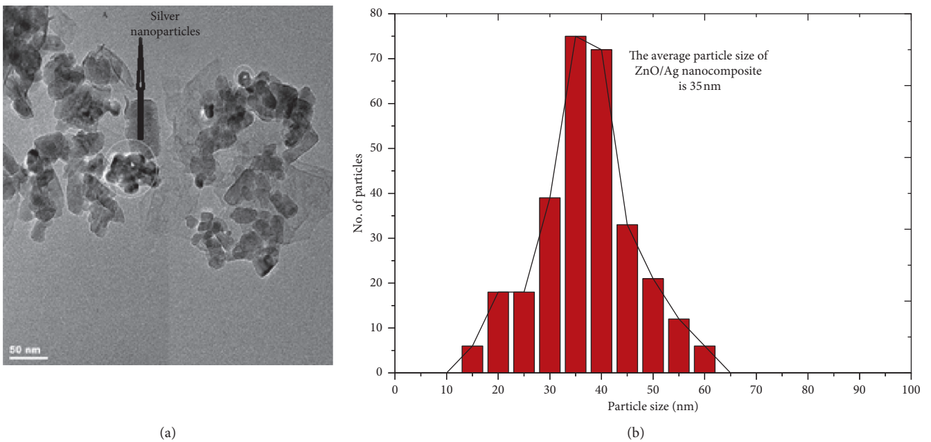
FIGURE 4: (a) TEM micrograph of ZnO/Ag. (b) Particle size distribution of ZnO/Ag nanocomposite.
