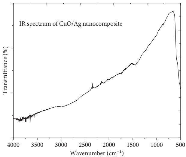
FIGURE 9: FTIR spectra analysis of CuO/Ag nanocomposite.
