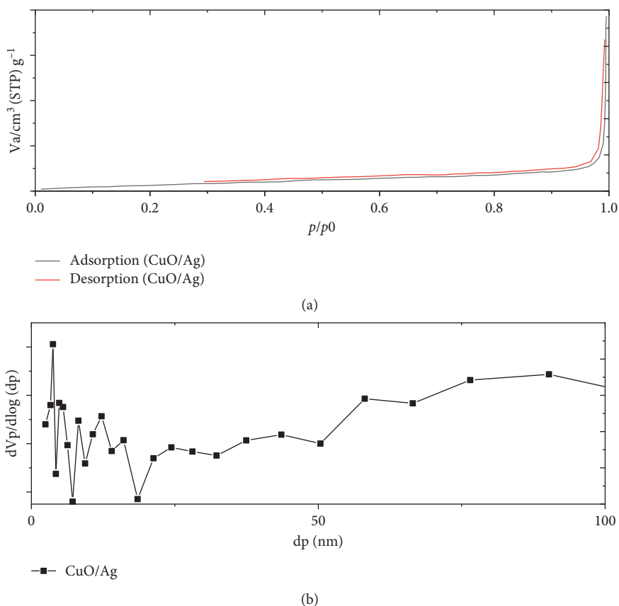
FIGURE 7: (a) Adsorption-desorption isotherms of nitrogen gas at 77 K and associated (b) BJH plot showing the pore size distribution of CuO/Ag.
