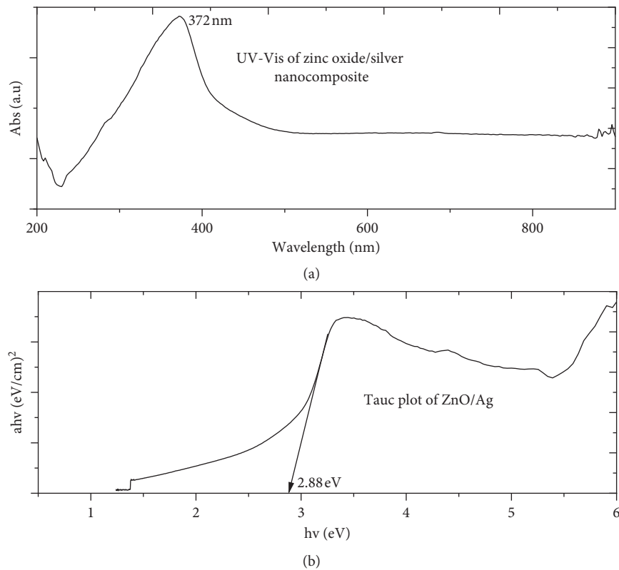
FIGURE 6: UV-Vis spectra of ZnO/Ag nanocomposite with its equivalent plot showing its energy band gap.
