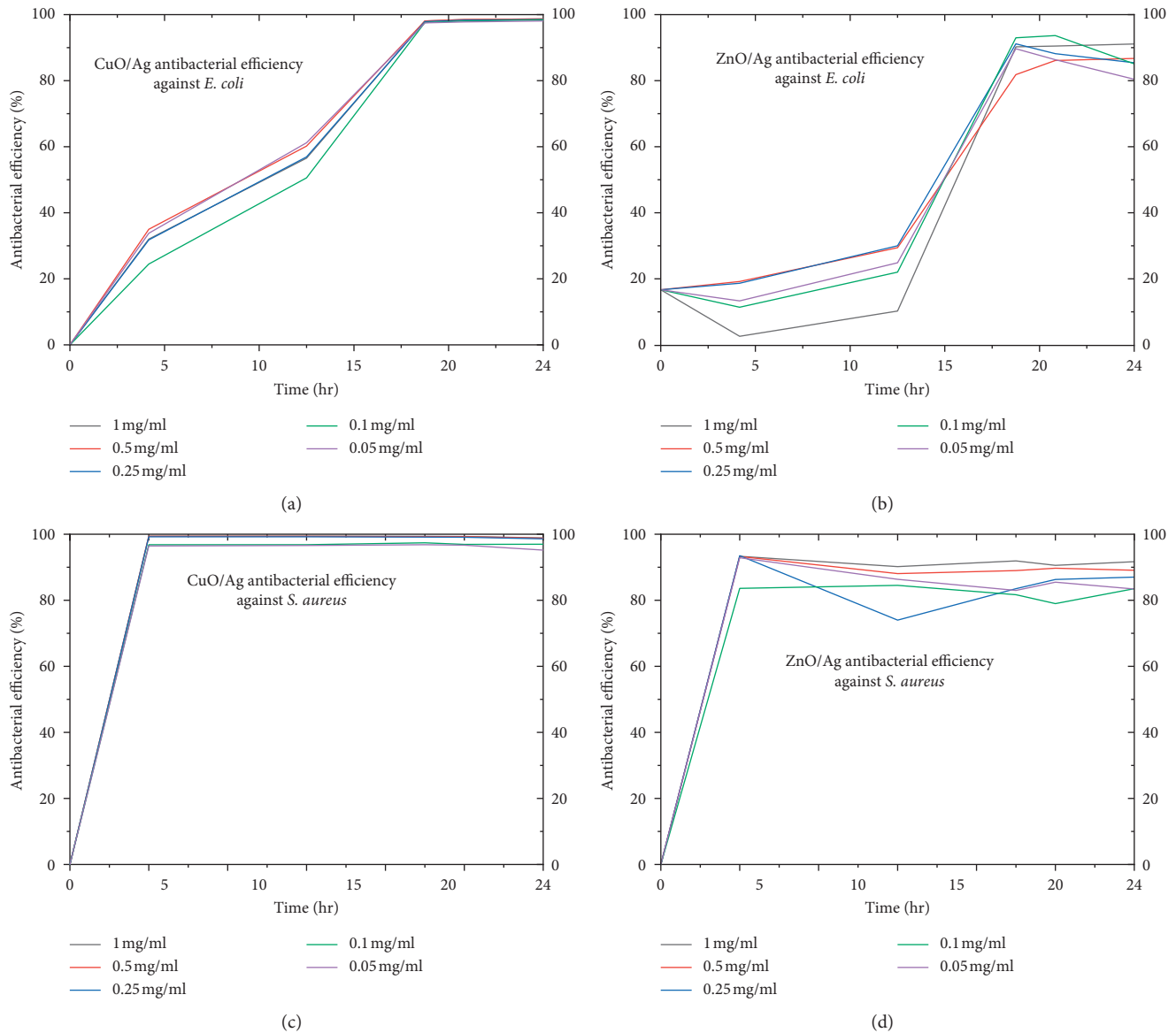
FIGURE 20: Kinetic growth study on E. coli and S. aureus that are alive after antibacterial activity by (a) CuO/Ag against E. coli , (b) ZnO/Ag against E. coli , (c) CuO/Ag against S. aureus , and (d) ZnO/Ag against S. aureus .
